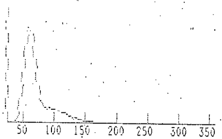
RBC HISTOGRAM
