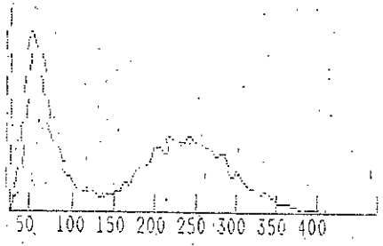
WBC HISTOGRAM
